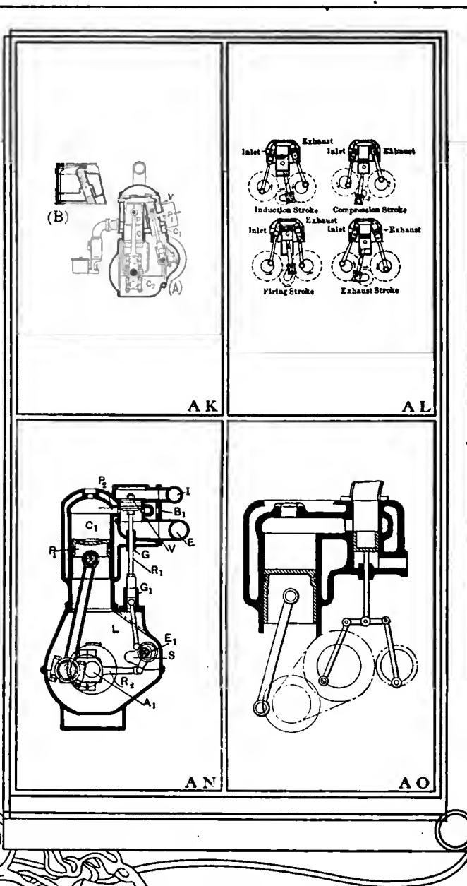
AJ—Bingham motor with piston valves, operated directly from below AK—Section of Hewitt piston valve motor AL—Diagram showing cycle of operations of Hewitt piston valve motor AO—Section of Pieper piston-valve motor AM—(A), Smith single-piston valve motor. (B), plan section of Smith motor, showing working and valve cylinders AN—Mann piston valve motor shown, single piston for intake and exhaust
